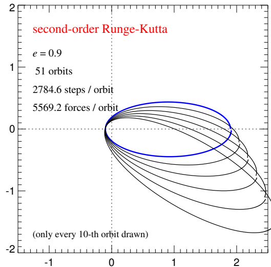
Figure 1: Kepler orbit
