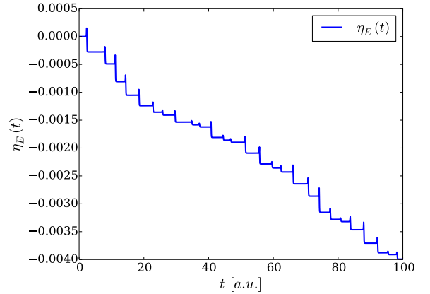
(b) Fourth-order accuracy
