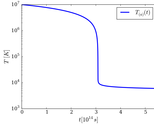
Figure 1: Second-order Runge-Kutta temperature evolution
