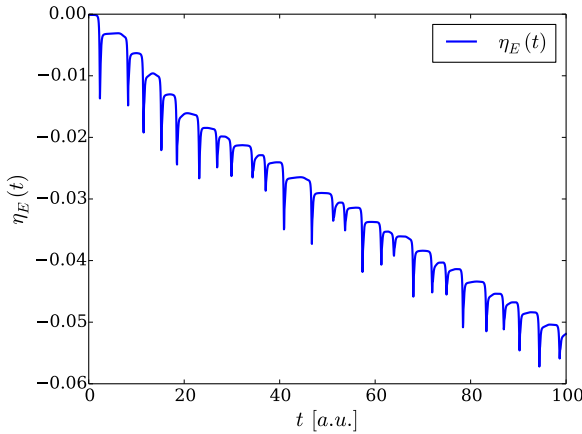
(a) Second-order accuracy
