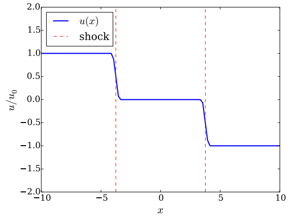
(b) Sketch of u(x)
