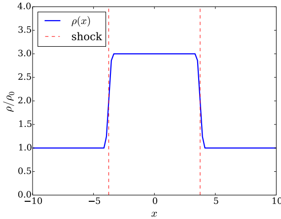
(a) Sketch of \rho(x)
