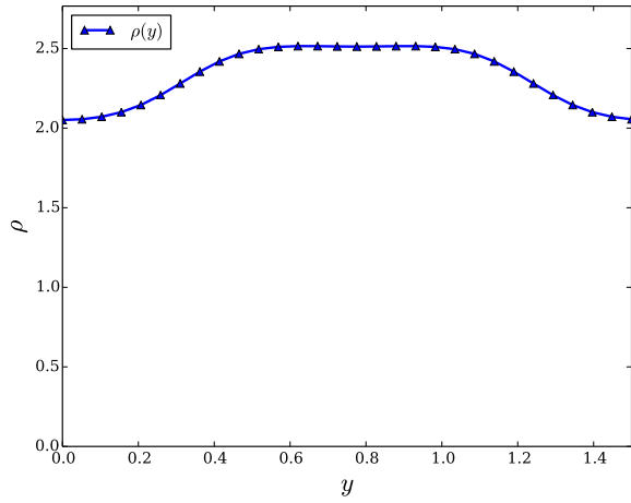
(a) \rho(y) for constant x
