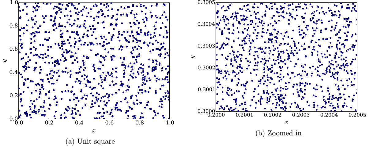
Figure 2: Scatter plots of 1000 points generated using the drand48 algorithm
