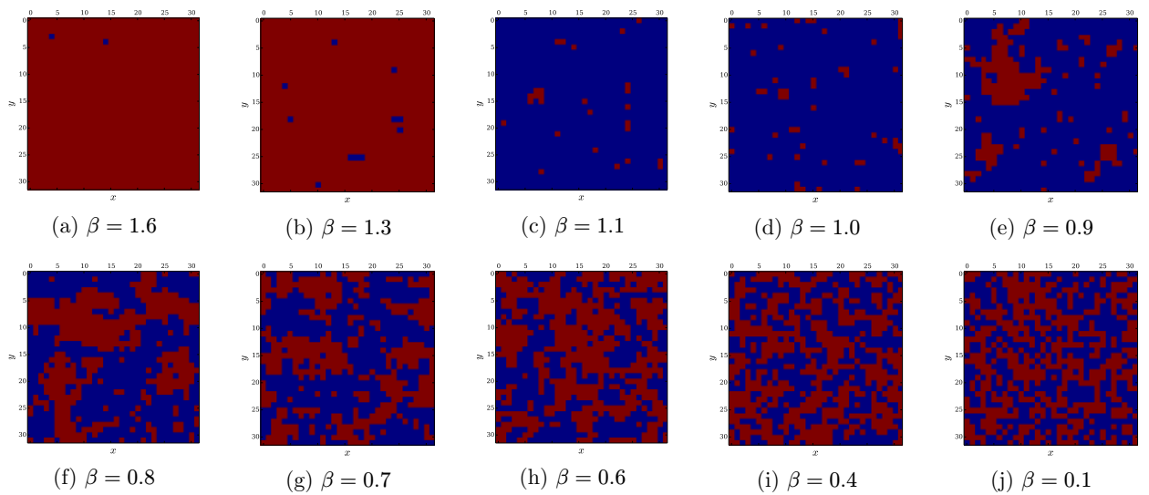
Figure 6: Color-coded (red: s_x = 1 , blue: s_x = -1 ) lattice configurations at different temperatures after 3000 relaxation sweeps
