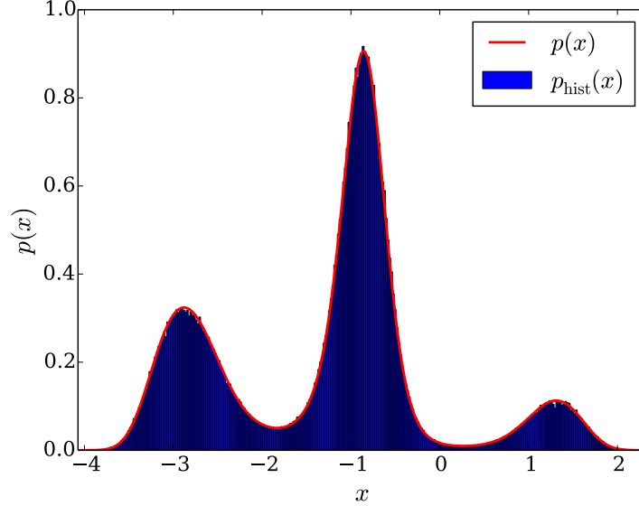
Figure 4: Histogram of points in a 10^6 -entry-long Markov chain, overplotted with the normalized target distribution function p(x)
