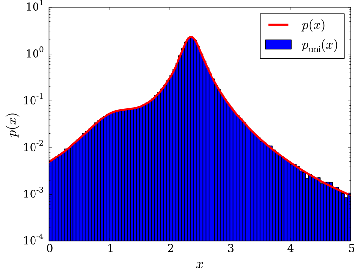
Figure 1: Histogram of accepted points, overplotted with the target distribution function p(x) (c) Figure 2 shows how the piecewise linear function f(x) envelopes the target distribution function p(x) . We clearly have f(x) \geq p(x) \forall x \in [0, 5] .
